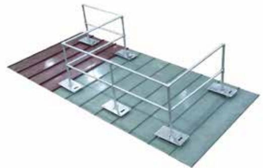
FitRite™ system on standing metal seam deck.
