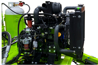
19 HP Isuzu Tier IV Diesel Engine
