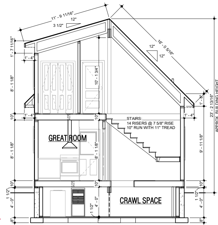
A 2 CROSS SECTION A 1/4" = 1'-0"
