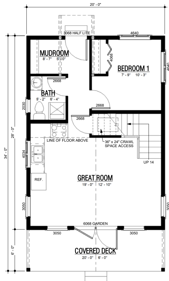
STUDY SET - MAIN 1/4" = 1'-0"
