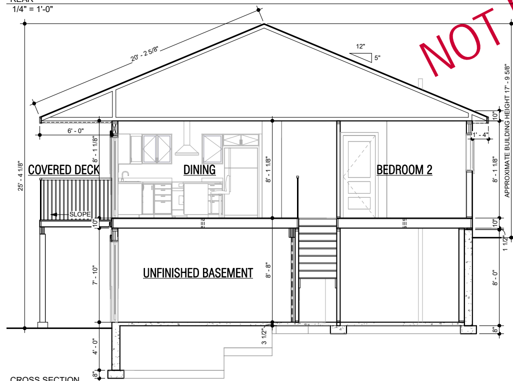
CROSS SECTION 1/4" = 1'-0"
