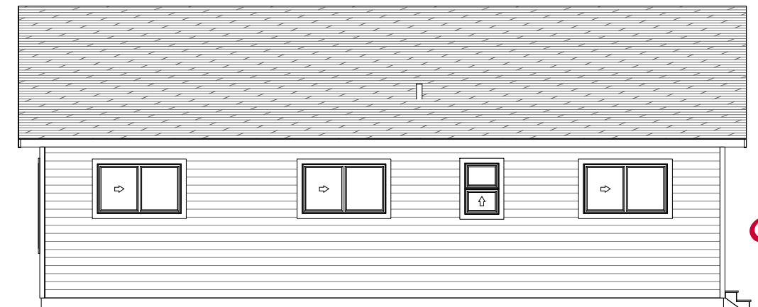
REAR 1/4" = 1'-0"
