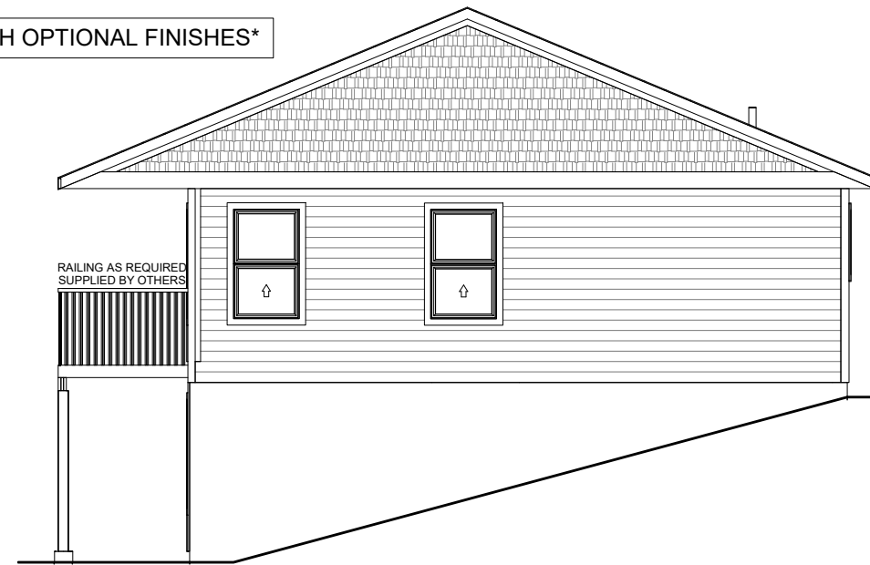
RIGHT 1/4" = 1'-0"
