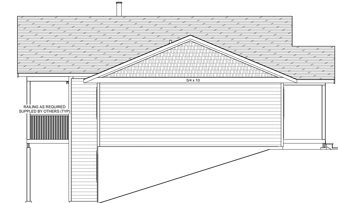
RIGHT 1/4" = 1'-0"
