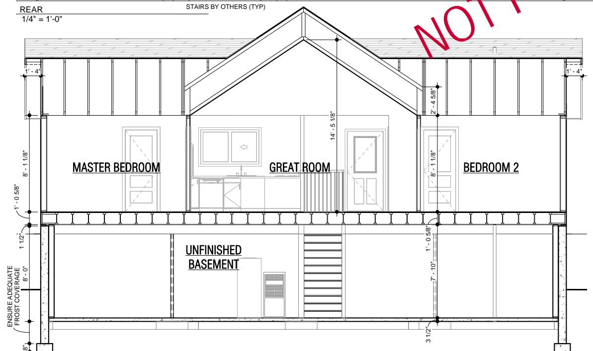
CROSS SECTION 1/4" = 1'-0"
