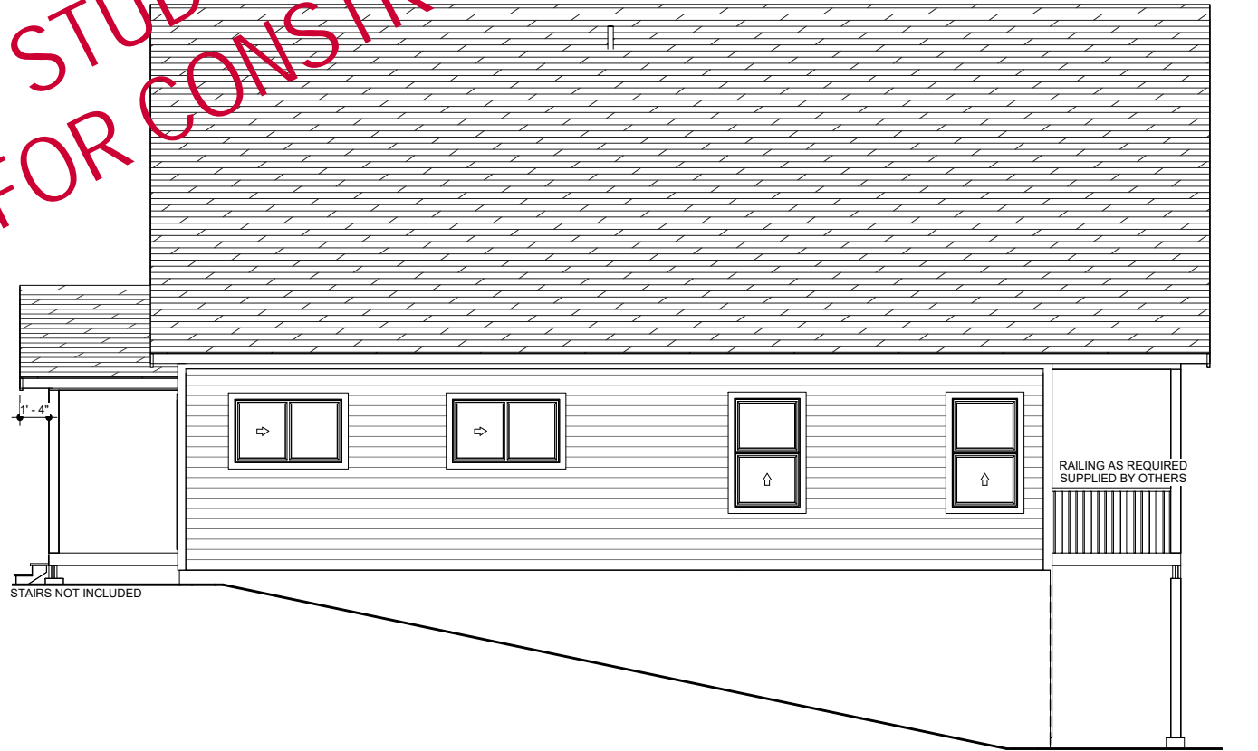
LEFT 1/4" = 1'-0"
