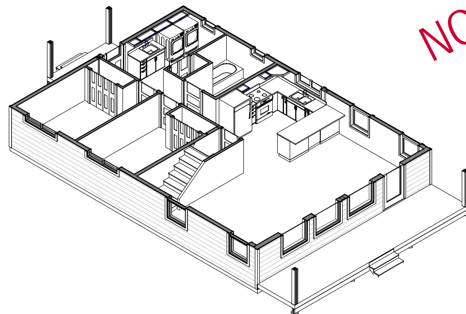
3D MAIN FLOOR
