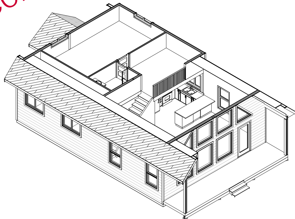
3D LOFT PLAN
