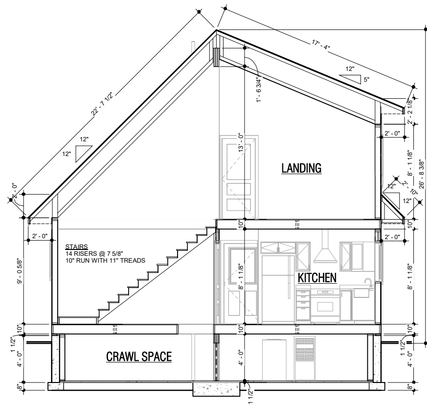
CROSS SECTION 1/4" = 1'-0"
